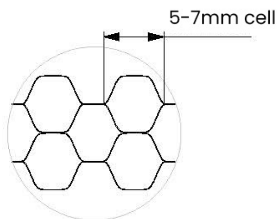
Cell detail
